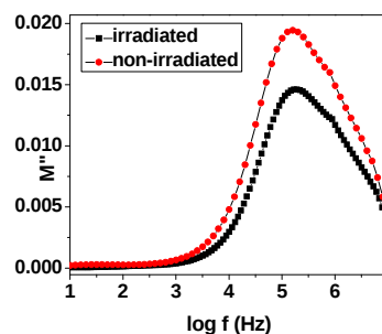
Figure 11. Plot of imaginary part of electric modulus versus log f for x = 40 mol% at 303K
