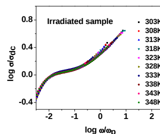
Figure 5. Plot of the scaled conductivity vs. normalized frequency for x = 40 mol%.
