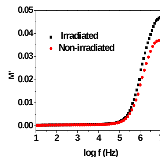
Figure 10. Plot of real part of electric modulus versus log f for x = 50 mol% at 303K
