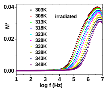
Figure 9. Frequency dependent real part of modulus at different temperatures for x = 40 mol%
