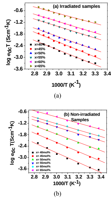
Figure 3. dc conductivity plots for different glass compositions
