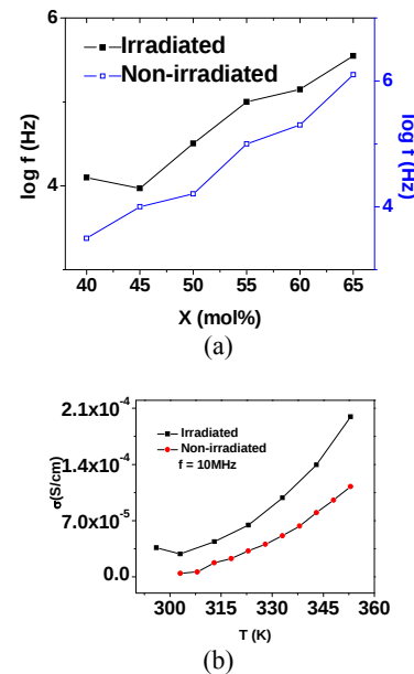
Figure 4. (a) Plot of relaxation frequency at 303K composition-wise at 303K; (b) Temperature dependence of conductivity at 10 MHz for x = 50 mol%
