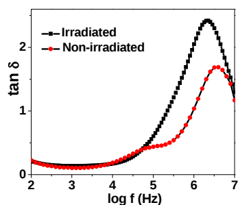
Figure 8. Variation of \tan \delta with frequency for x = 65 mol% at 303K
