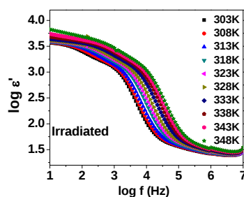
Figure 7(a). Frequency dependent dielectric constant at different temperatures for x = 40 mol%
