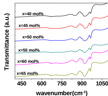
Figure 2. IR spectra of irradiated glass samples at room temperature
