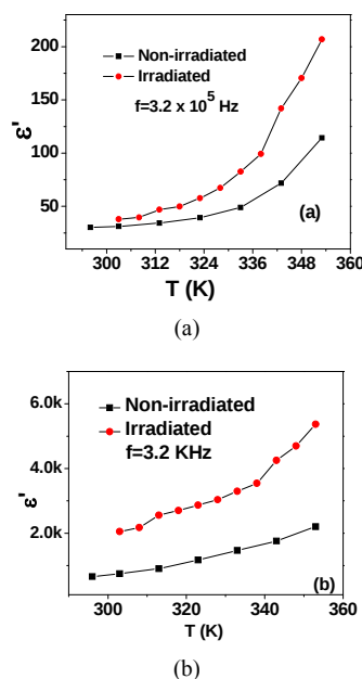
Figure 6(a). Variation of dielectric constant with temperature at 3.2 \times 10^5 Hz and & Figure 6(b) at 3.2 \times 10^3 Hz respectively for x = 45 mol%
