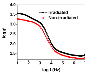
Figure 7(b) the frequency dependence of dielectric constant for x = 40 mol% at 303K
