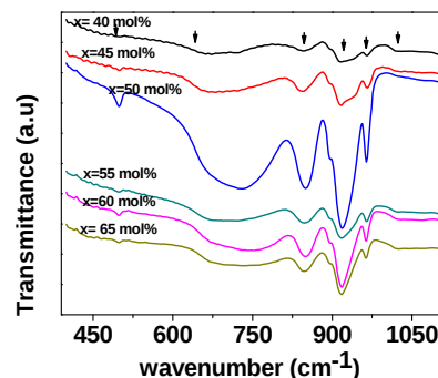
Figure 1. Infrared spectra of non-irradiated glass samples at room temperature
