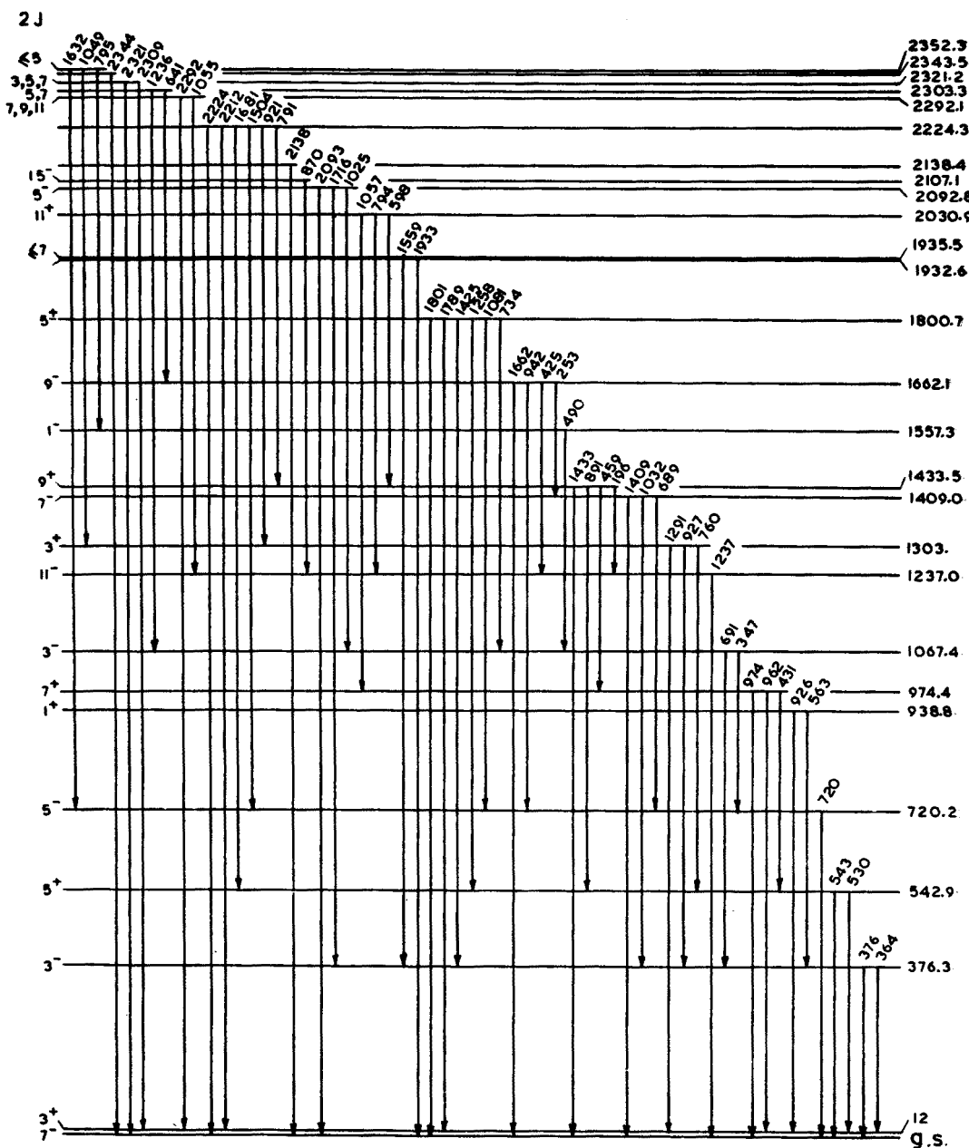
Fig. 4. Partial decay scheme of ^{45}\text{Sc} observed in the present experiment. Spin values given are 2J and level energies are in keV
