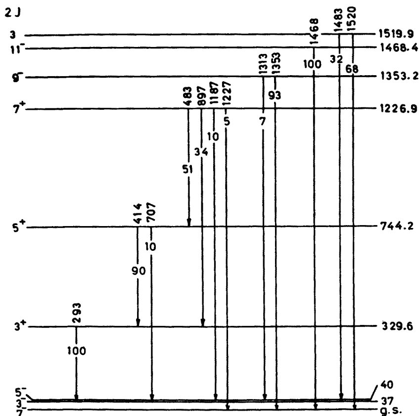
Fig. 5. Partial decay scheme of ^{45}\text{Ti} observed in the present experiment + spin values are given as 2J and energies in keV
